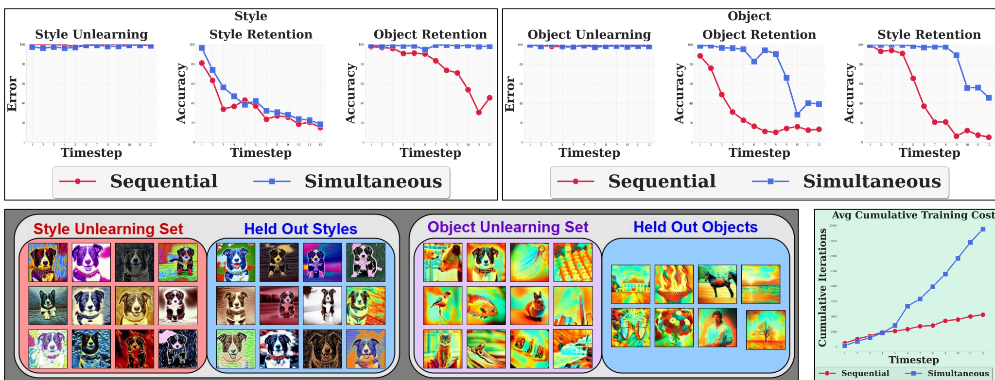
Unlearning Requests Arrive Sequentially
