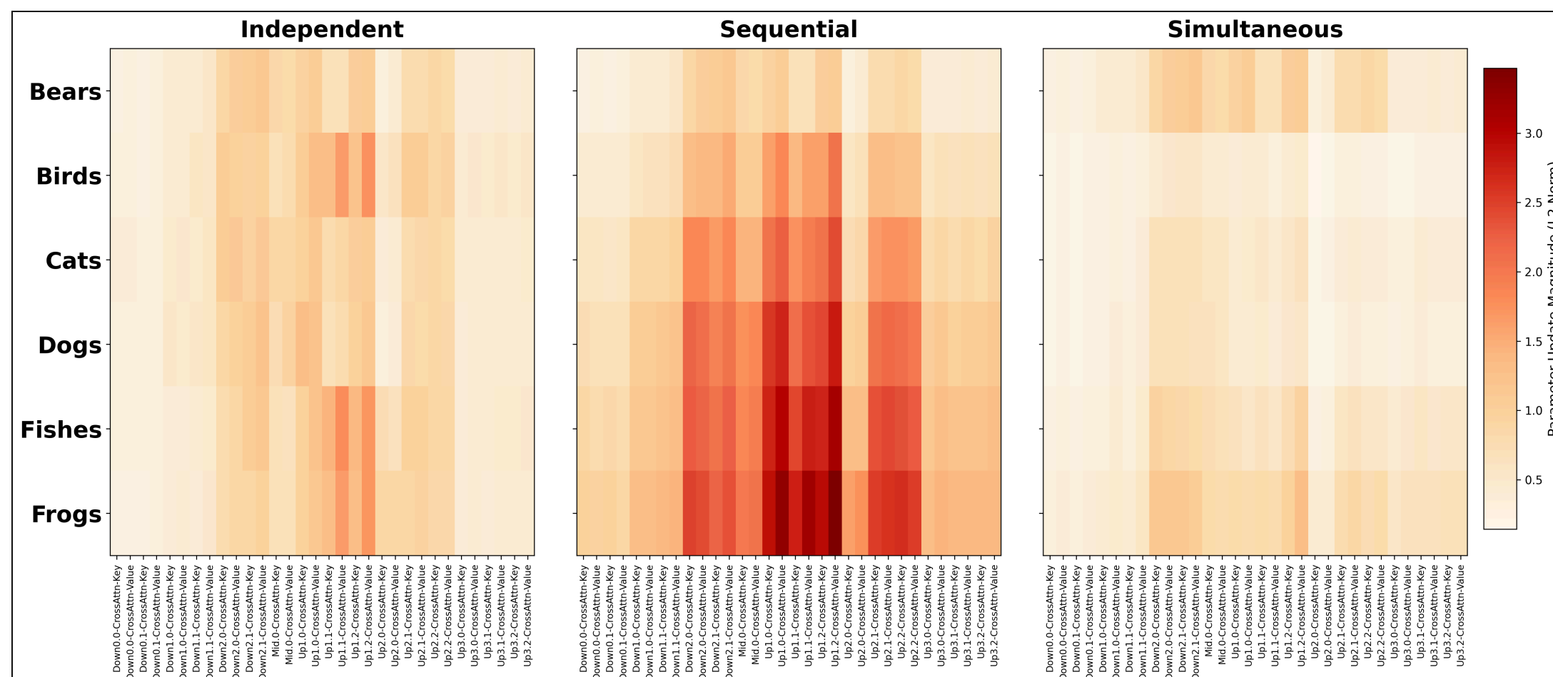
Simultaneous Unlearning uses smaller parameter updates
